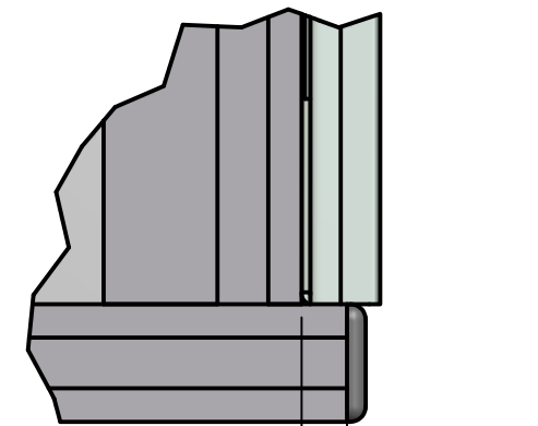
DETAIL A SCALE .75
